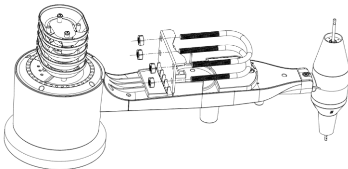
Figure 3: U-Bolt installation
