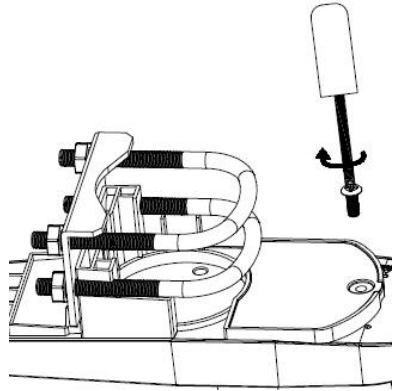
Figure 7: Battery installation diagram
