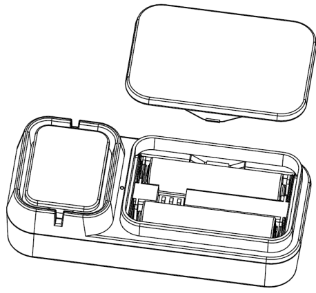
Figure 2: Battery installation
