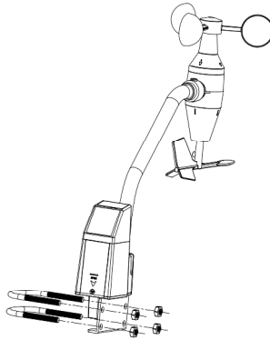
Figure 2: U-Bolt installation
