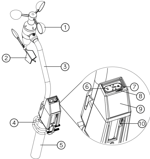
Figure 1: Sensor assembly components
