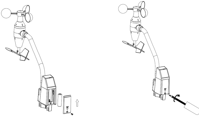
Figure 6: Battery installation diagram
